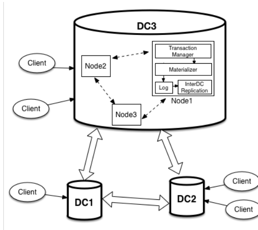
Figure 1 – Cure's Architecture
